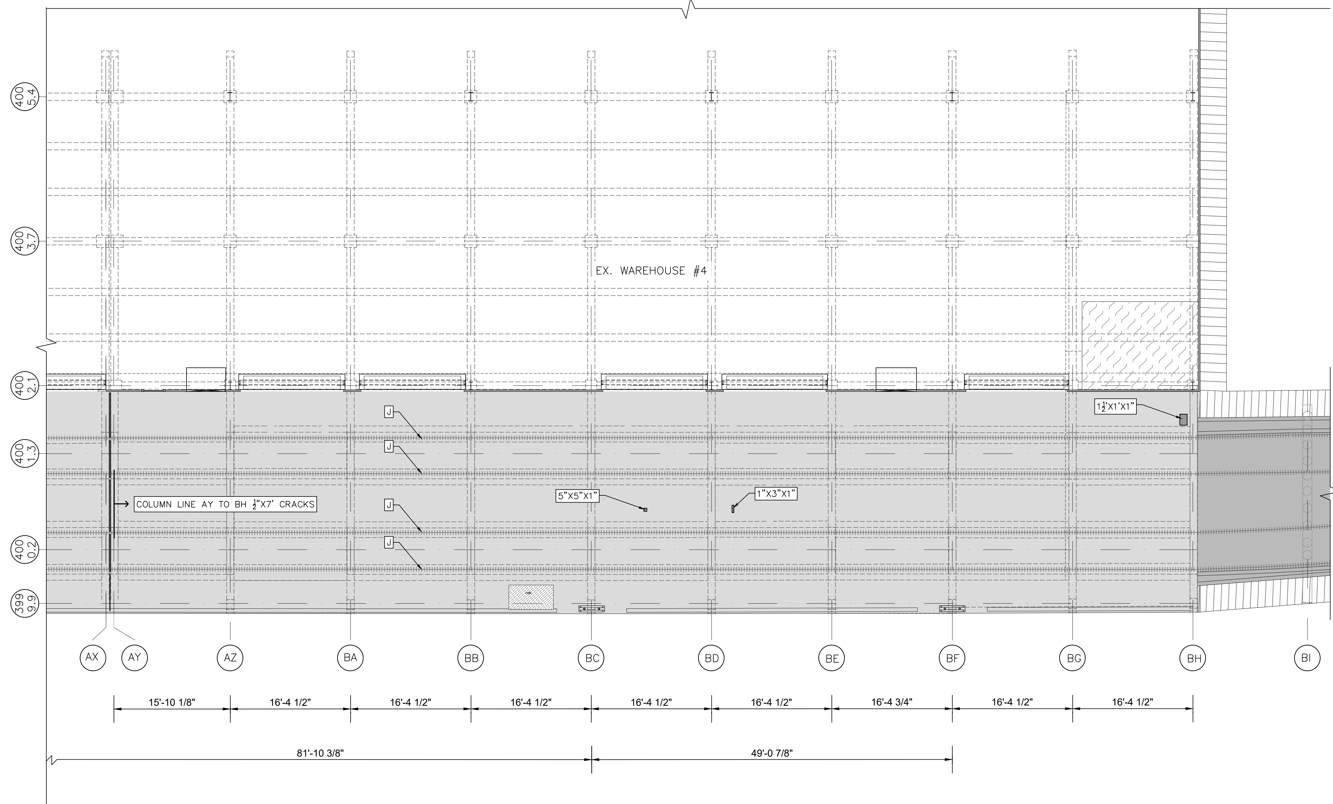
1 S-4.1 BERTH SURFACE REPAIR PLAN 4 SCALE: 1/8"=1'
